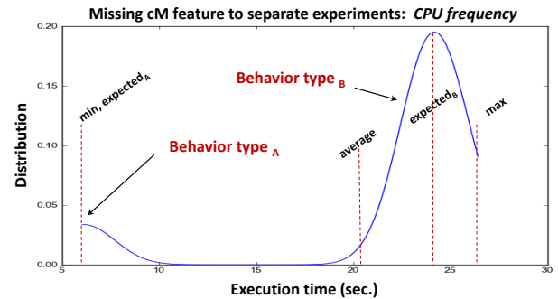
Fig. 15. Unexpected behavior helped to identify and add a missing feature to cM (processor frequency) as well as software dependency (cpufreq) that ensures reproducibility of experimental results.
